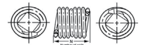
Self-Locking Insert
