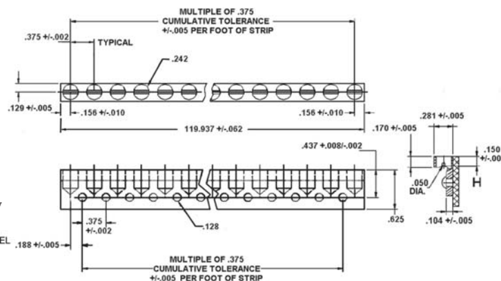
Typical Assembly
