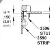
Typical Assembly
