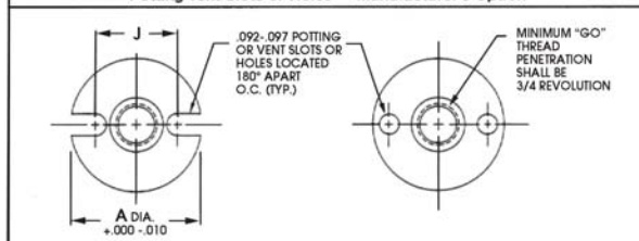
Potting Vent Slots or Holes — Manufacturer's Option
